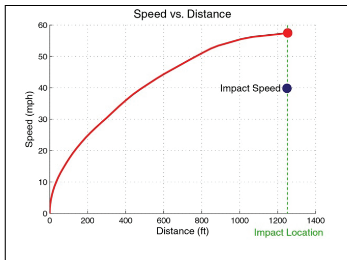
Figure 16: Speed without braking
