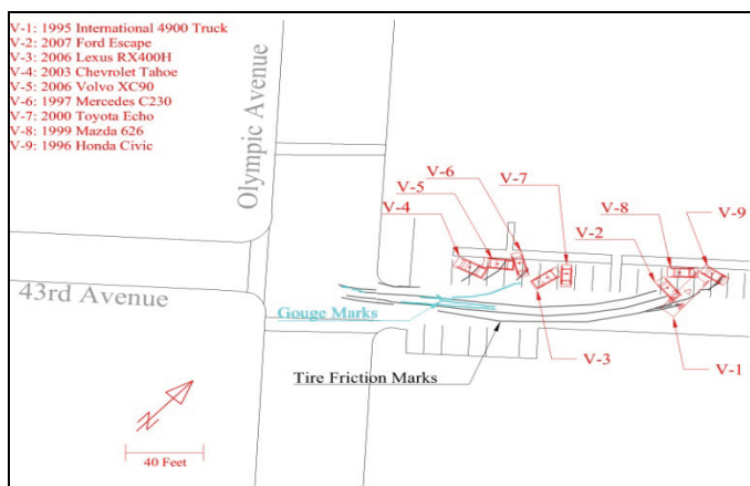
Figure 4: Computer drawing of scene, vehicle rest positions, and physical evidence
